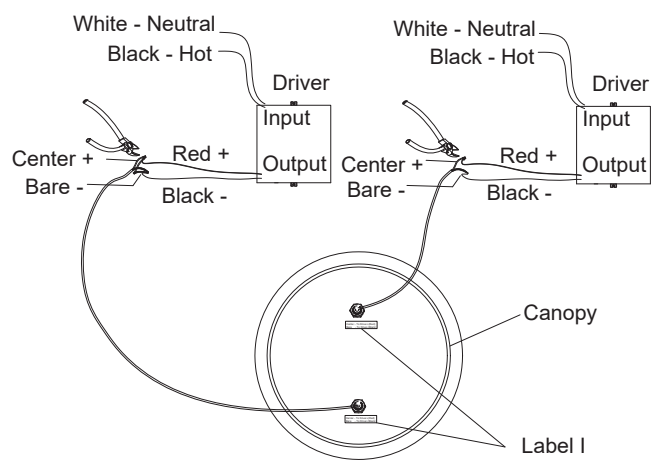
Fig.3 Driver Wires
